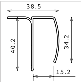
A PARED - FREE 2
